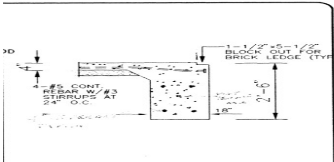
TYPICAL PERIMETER GRADE BEAM
