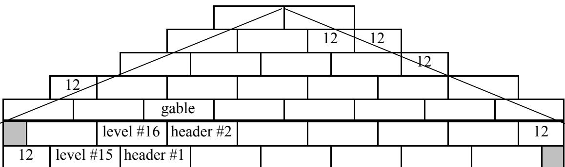
Rear wall view including gable from inside-facing rear wall
